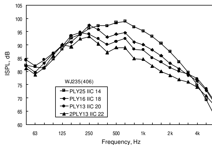
Figure 28: Normalized impact sound pressure levels for three thicknesses of plywood and a double sheet of 13 mm plywood.
