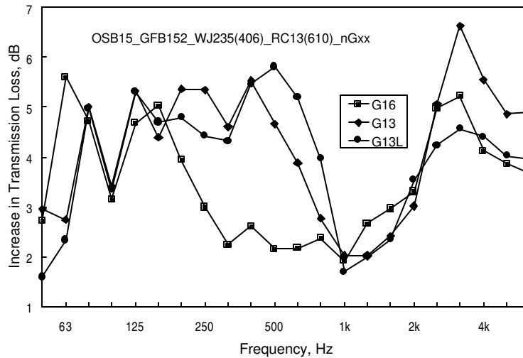
Figure 37: Increase in TL caused by adding a second layer of gypsum board.
