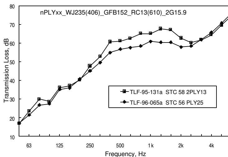
Figure 35: TL plots showing effect of changing sub-floor from one layer of 25 mm thick plywood to two layers of 13 mm plywood.
