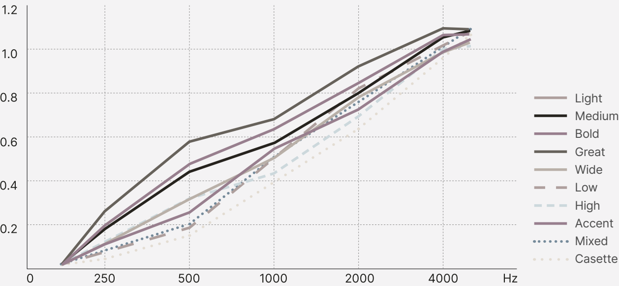
Absorption Coefficient for: no gap, 9mm 1900 g/m 2
