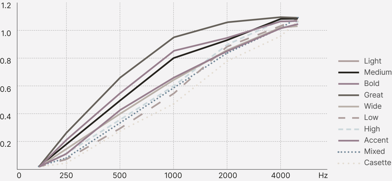
Absorption Coefficient for: 200 mm gap, 9mm 1900 g/m 2
